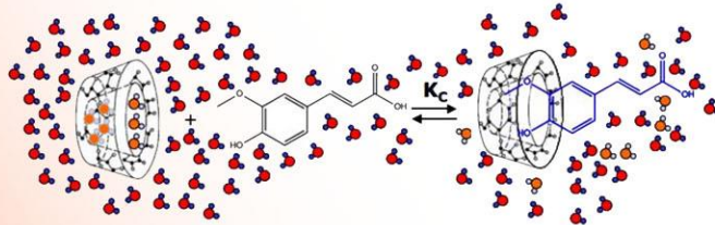
Hydroxypropyl Cyclodextrin
