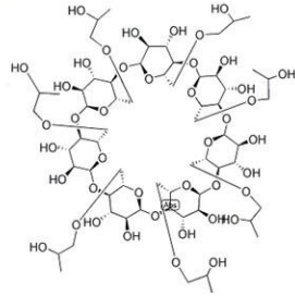
Hydroxypropyl Cyclodextrin
